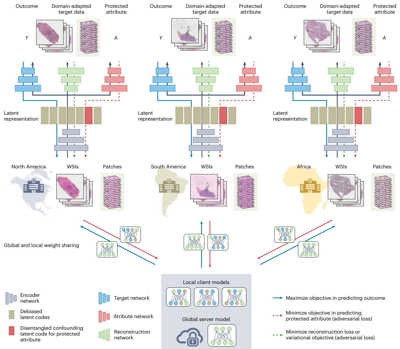
Fig. 5 | A decentralized framework that integrates federated learning with adversarial learning and disentanglement. In addition to aiding the development of algorithms using larger and more diverse patient populations, federated learning can be integrated with many techniques in representation learning and in unsupervised domain adaptation that can learn in the presence of unobserved protected attributes. In federated learning, global and local weights are shared between the global server and the local clients (such as different hospitals in different countries), each with different datasets of whole-slide images (WSIs) and image patches. Different domain-adaptation methods can be used with federated learning. In federated adversarial and debiasing (FADE), the client IDs were used as protected attributes, and adversarial learning was used to
